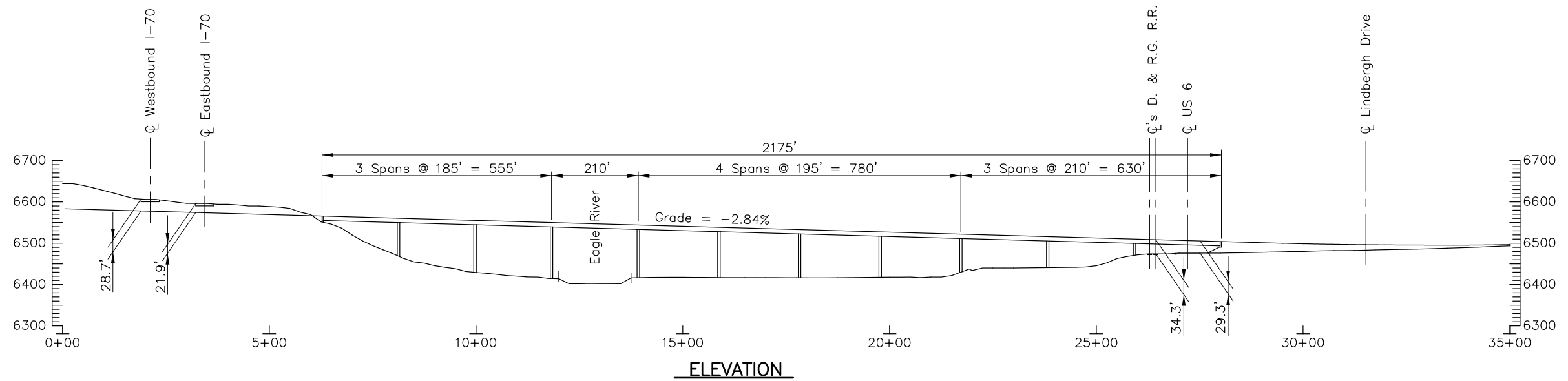
Figure 2-5 EAGLE AIRPORT INTERCHANGE ALTERNATIVE F MODIFIED
